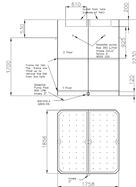
Flutningstankur
